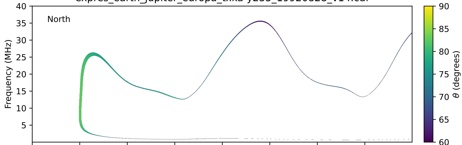
expres_earth_jupiter_europa_txka-y235_19920828_v14.cdf
