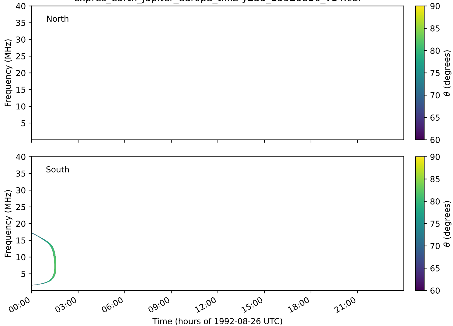
expres_earth_jupiter_europa_txka-y235_19920826_v14.cdf
