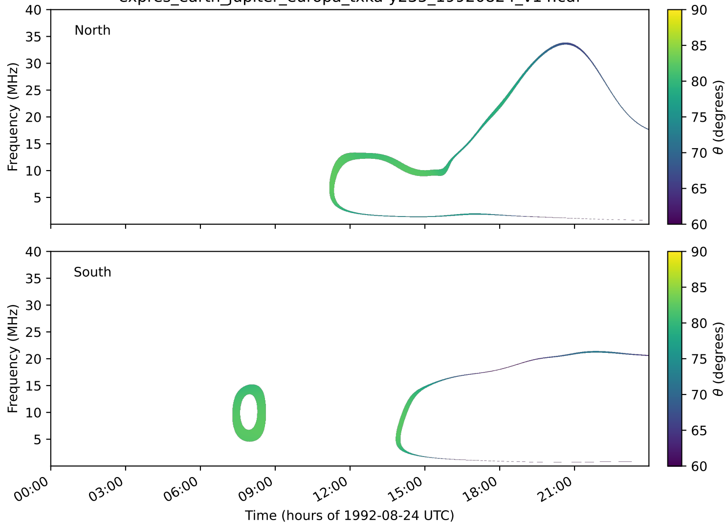
expres_earth_jupiter_europa_txka-y235_19920824_v14.cdf
