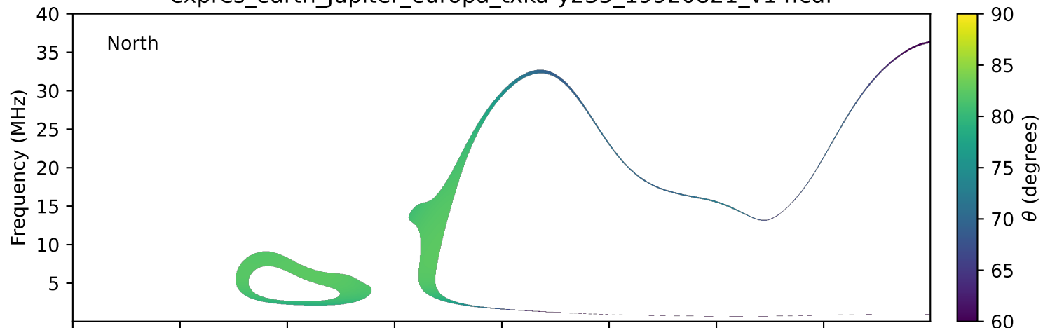
expres_earth_jupiter_europa_txka-y235_19920821_v14.cdf
