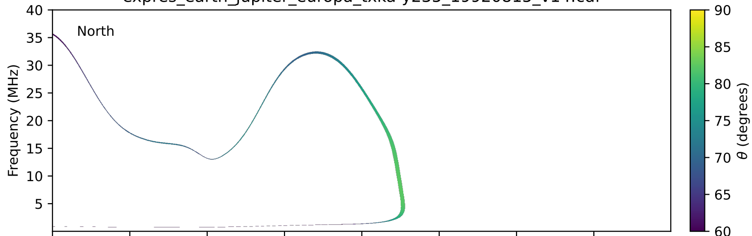
expres_earth_jupiter_europa_txka-y235_19920815_v14.cdf
