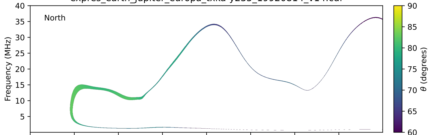
expres_earth_jupiter_europa_txka-y235_19920814_v14.cdf
