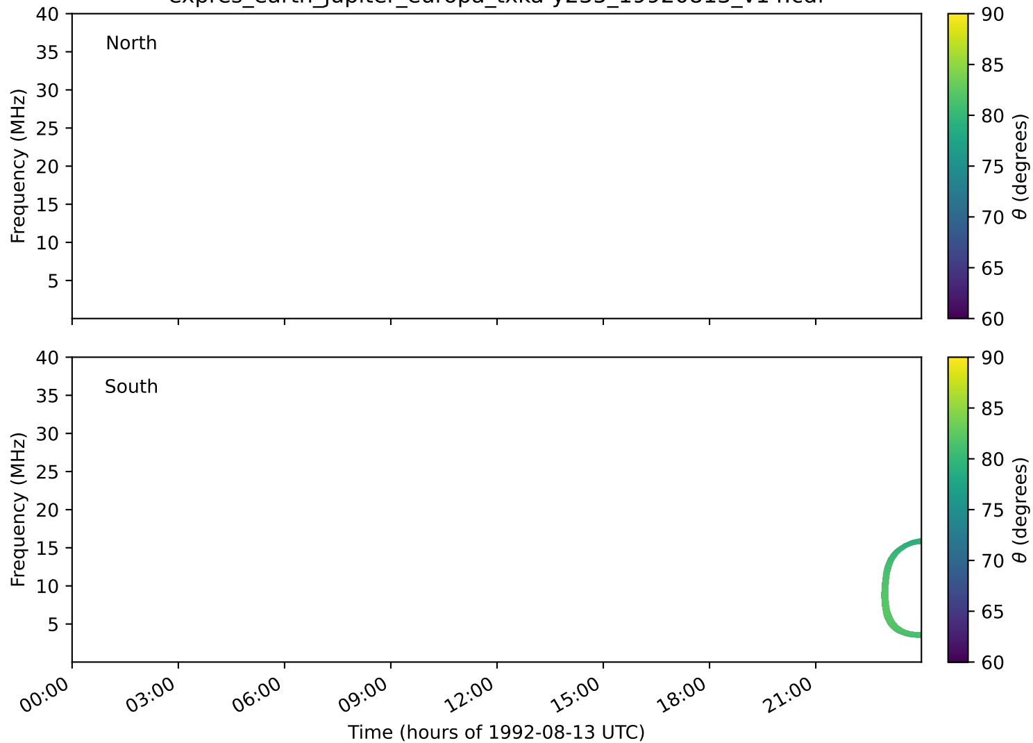
expres_earth_jupiter_europa_txka-y235_19920813_v14.cdf
