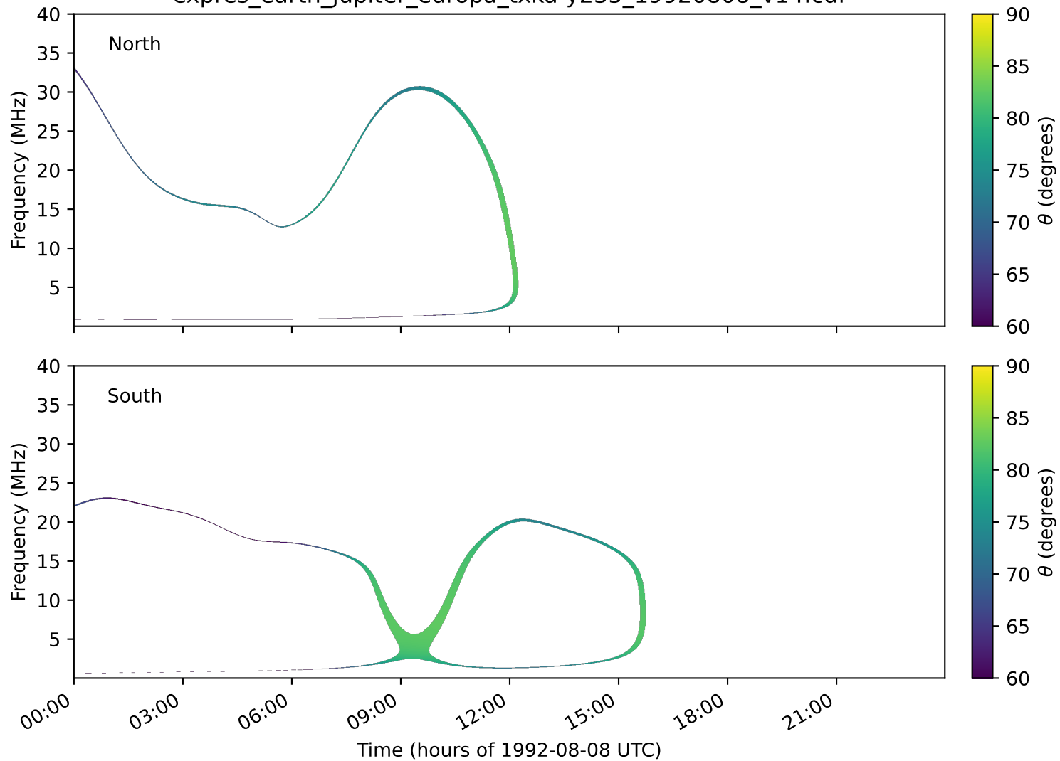
expres_earth_jupiter_europa_txka-y235_19920808_v14.cdf
