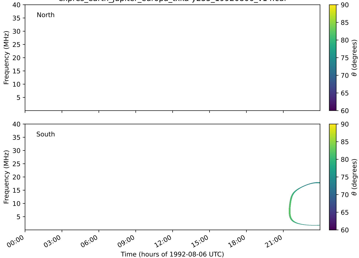
expres_earth_jupiter_europa_txka-y235_19920806_v14.cdf
