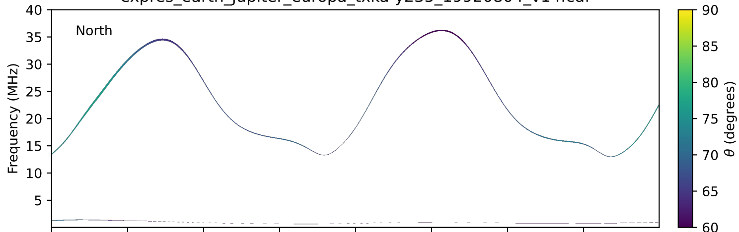
expres_earth_jupiter_europa_txka-y235_19920804_v14.cdf
