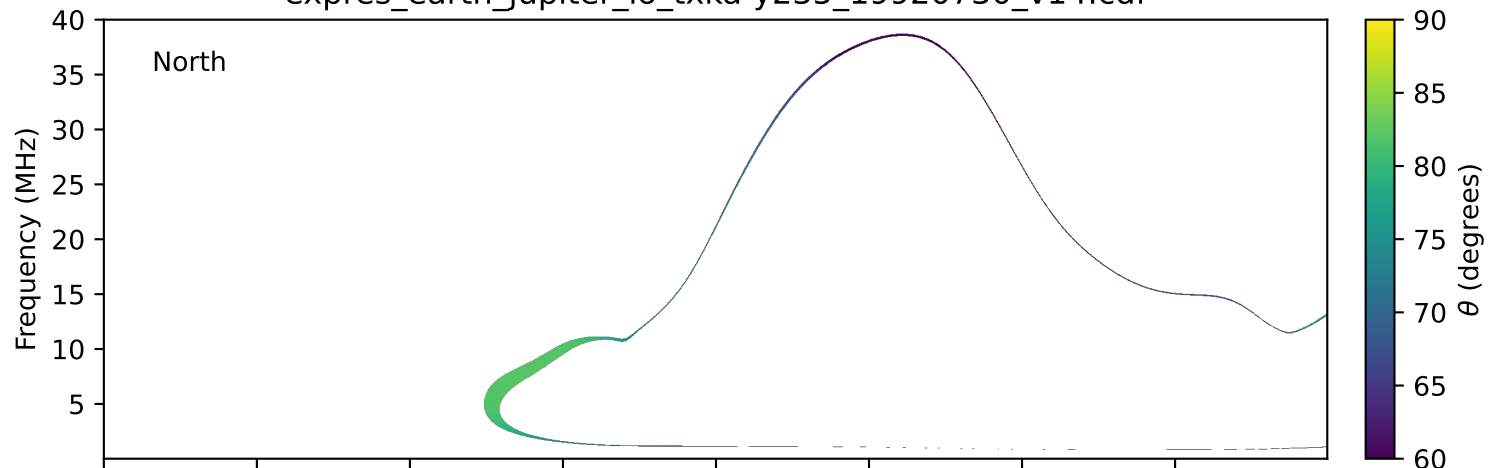
expres_earth_jupiter_io_txka-y235_19920730_v14.cdf
