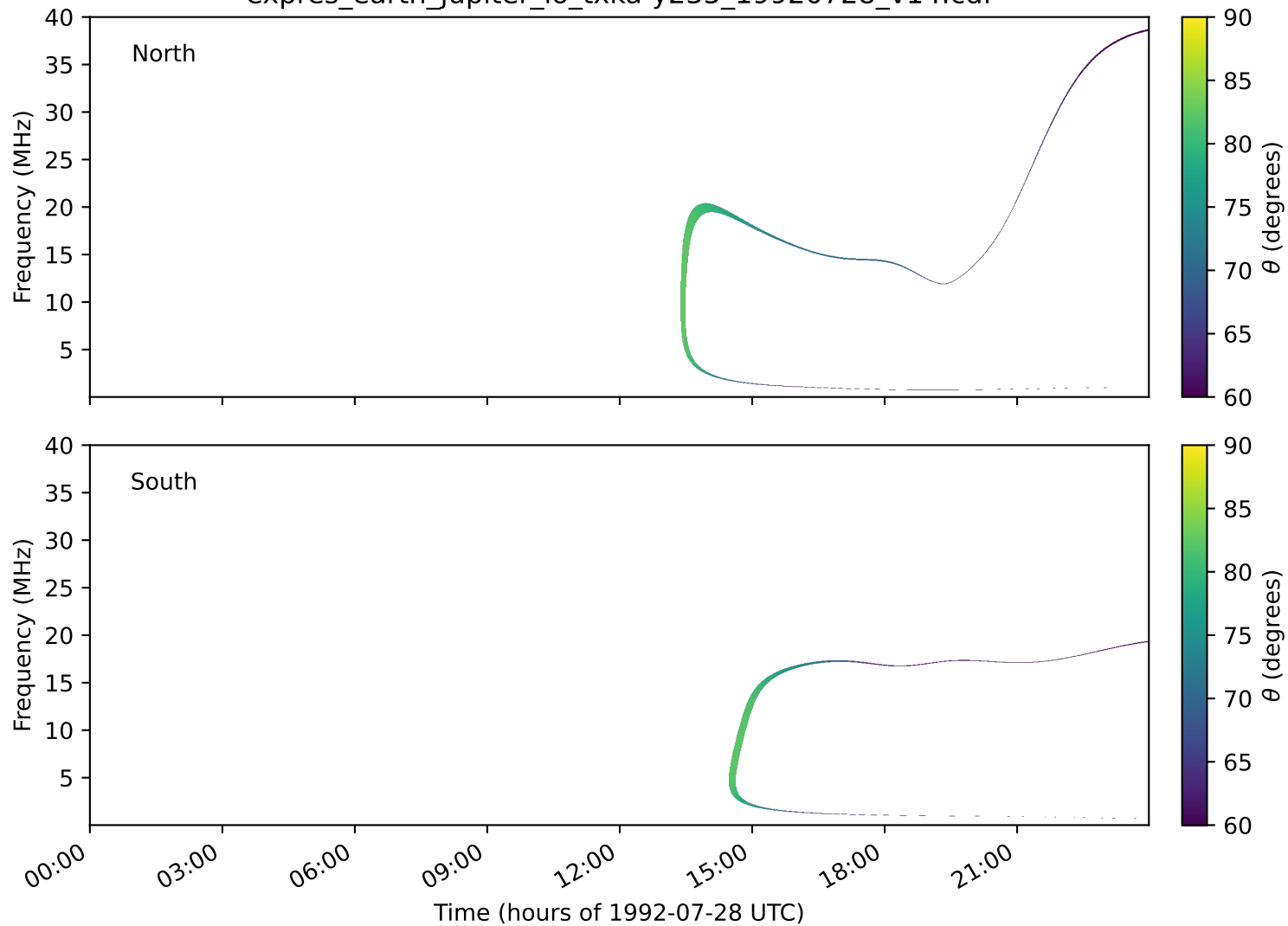
expres_earth_jupiter_io_txka-y235_19920728_v14.cdf
