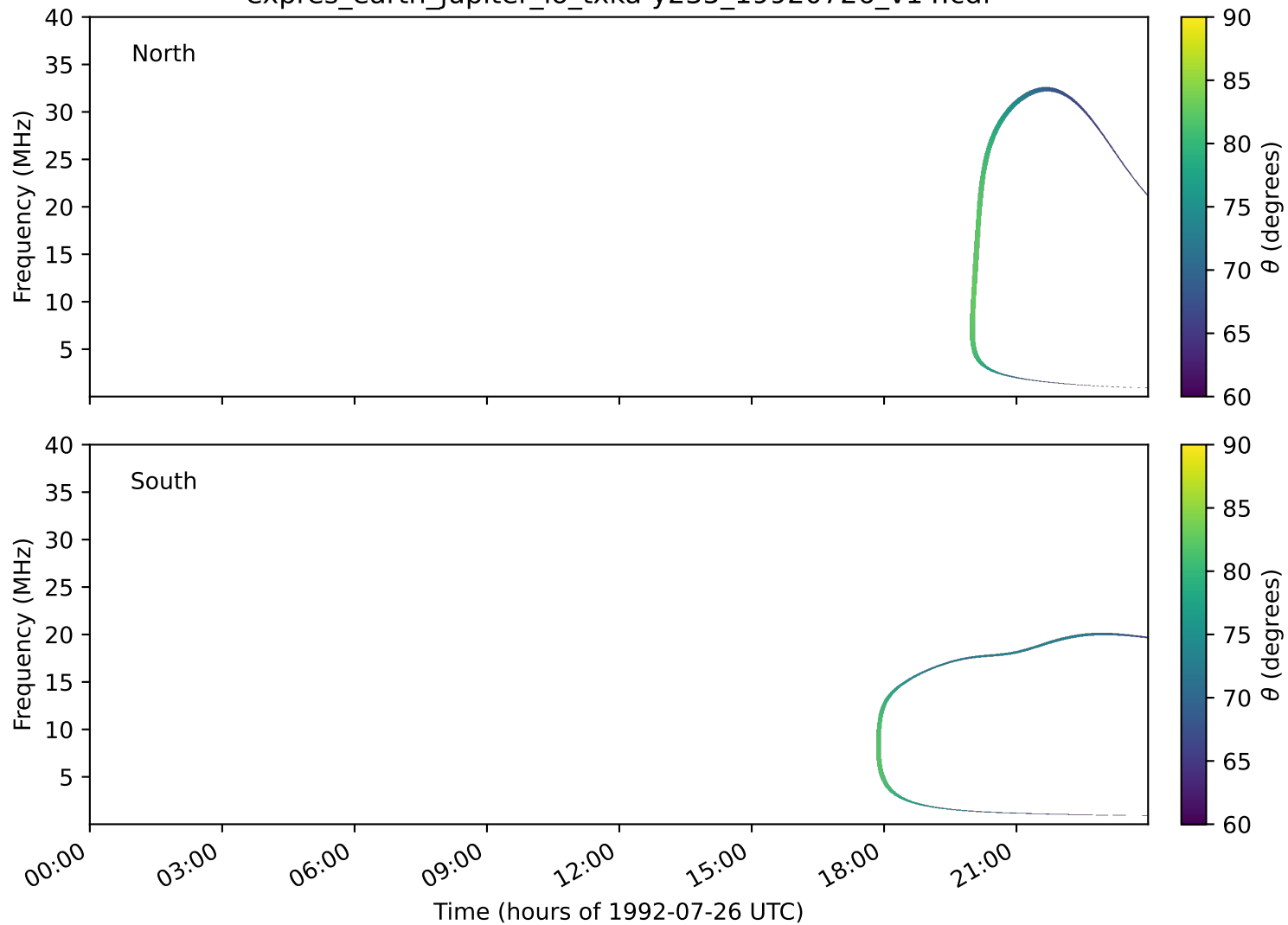
expres_earth_jupiter_io_txka-y235_19920726_v14.cdf
