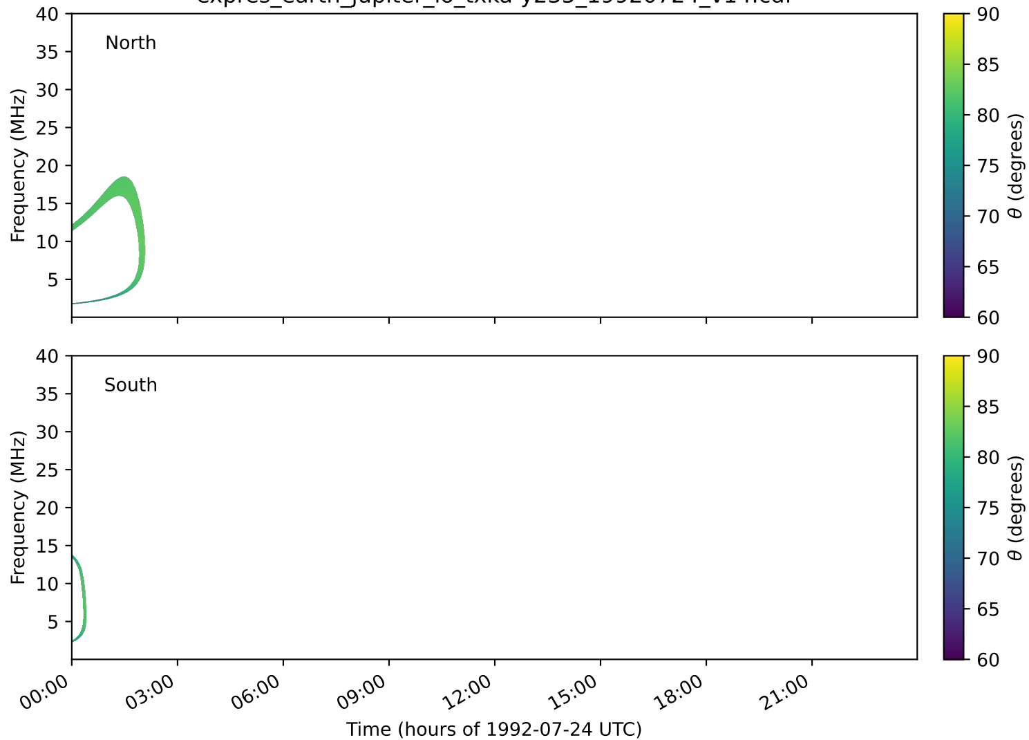
expres_earth_jupiter_io_txka-y235_19920724_v14.cdf
