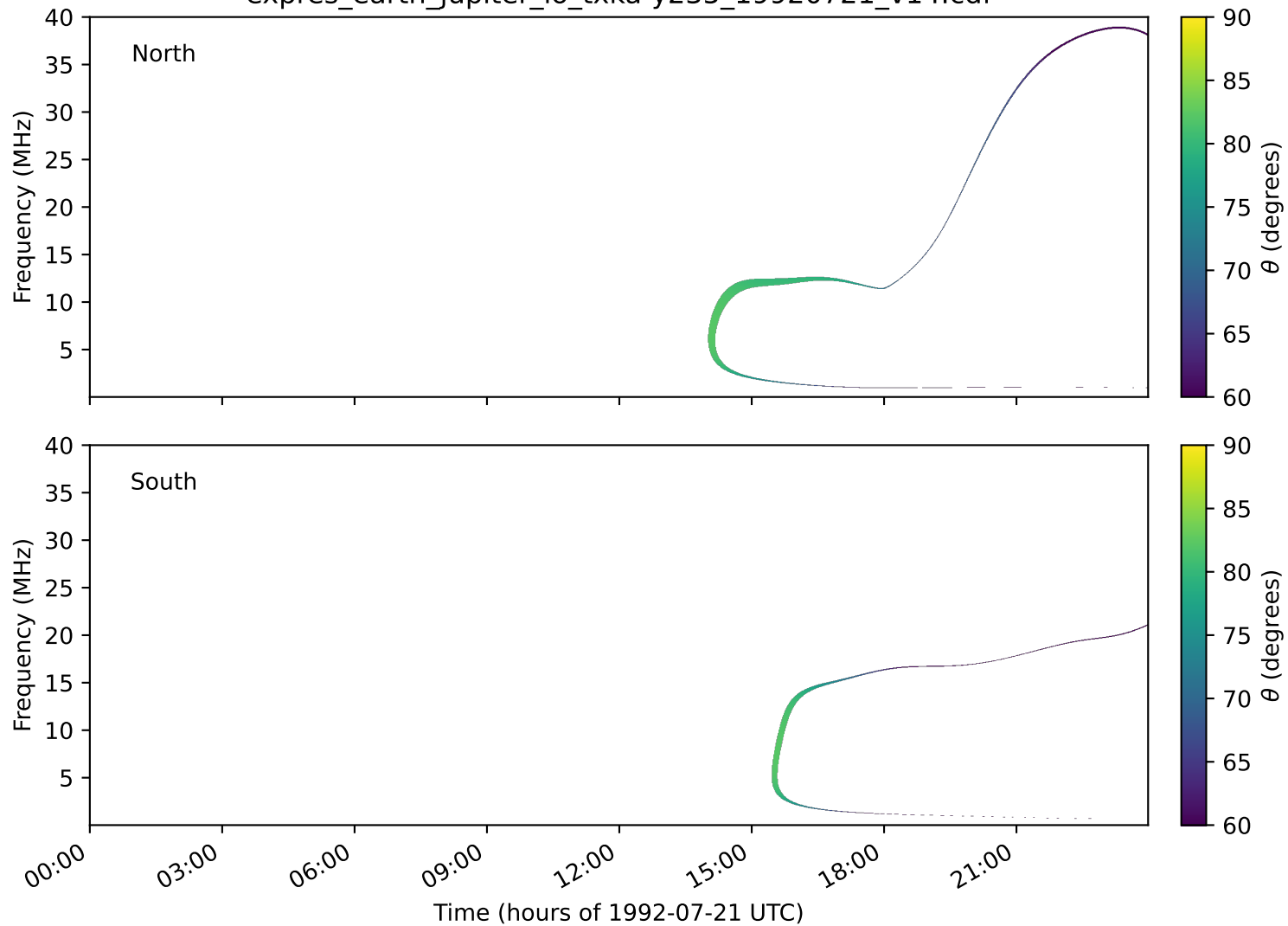
expres_earth_jupiter_io_txka-y235_19920721_v14.cdf
