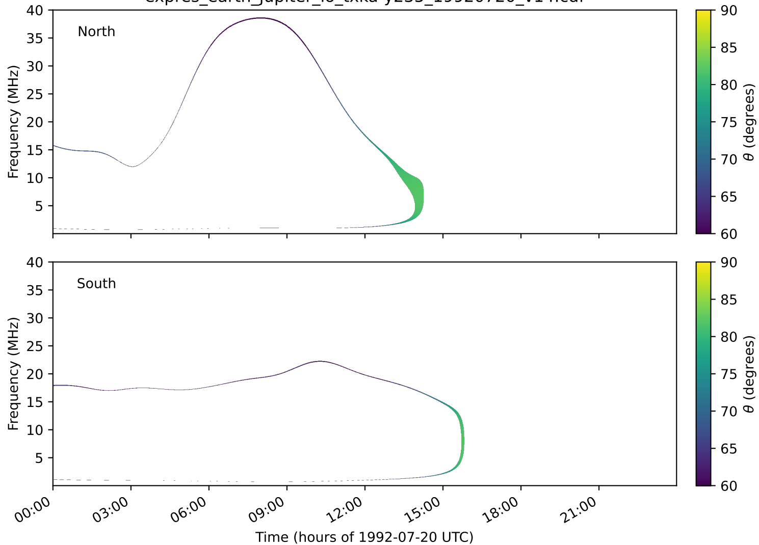
expres_earth_jupiter_io_txka-y235_19920720_v14.cdf
