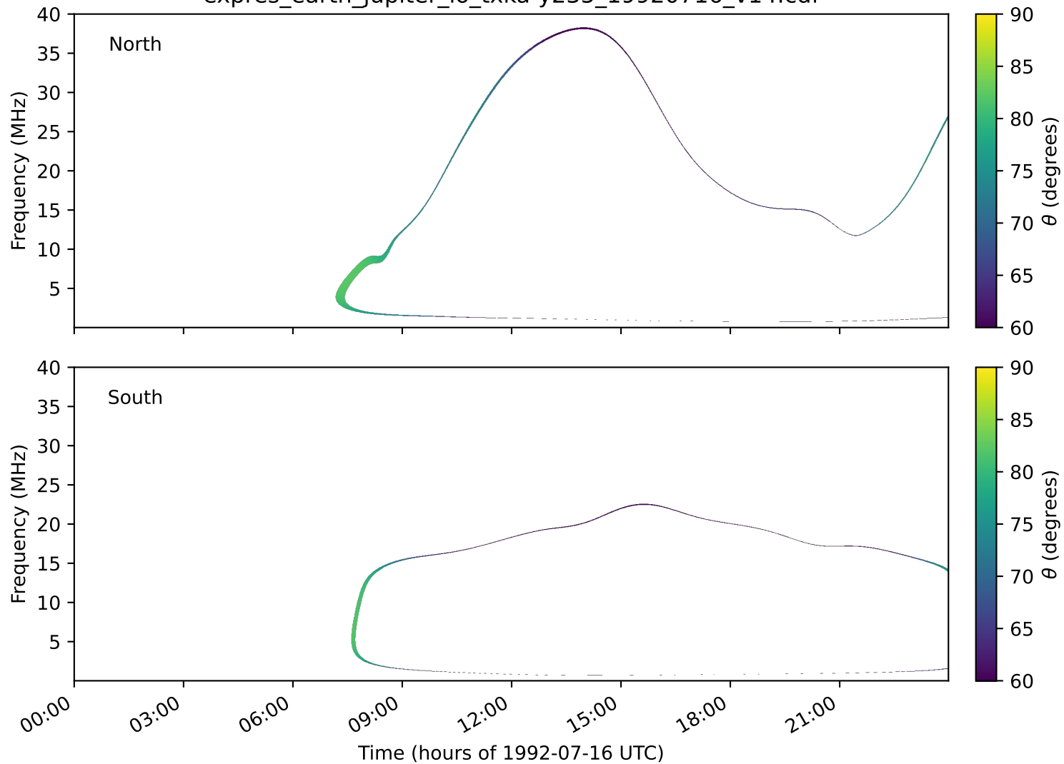
expres_earth_jupiter_io_txka-y235_19920716_v14.cdf
