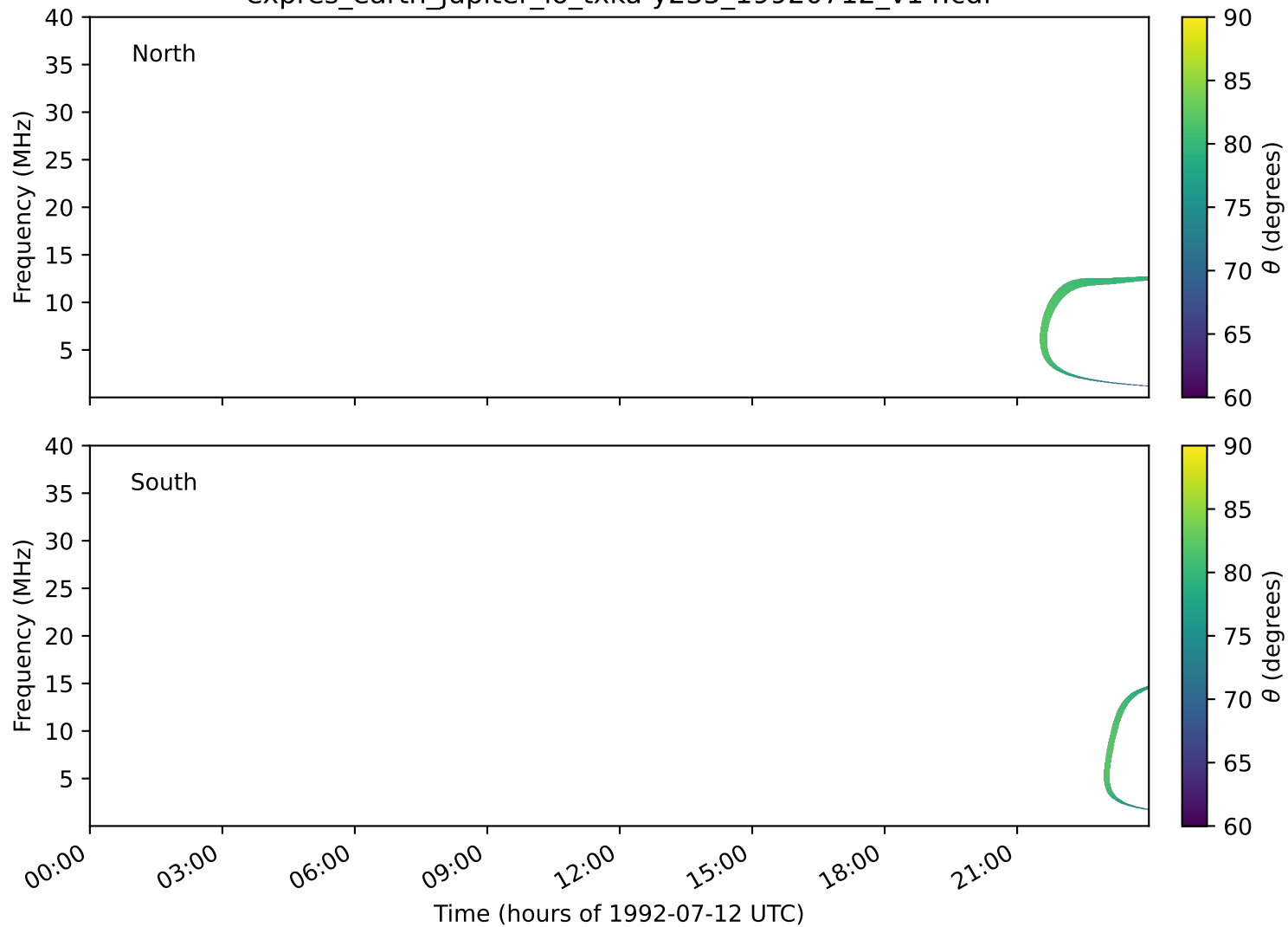
expres_earth_jupiter_io_txka-y235_19920712_v14.cdf
