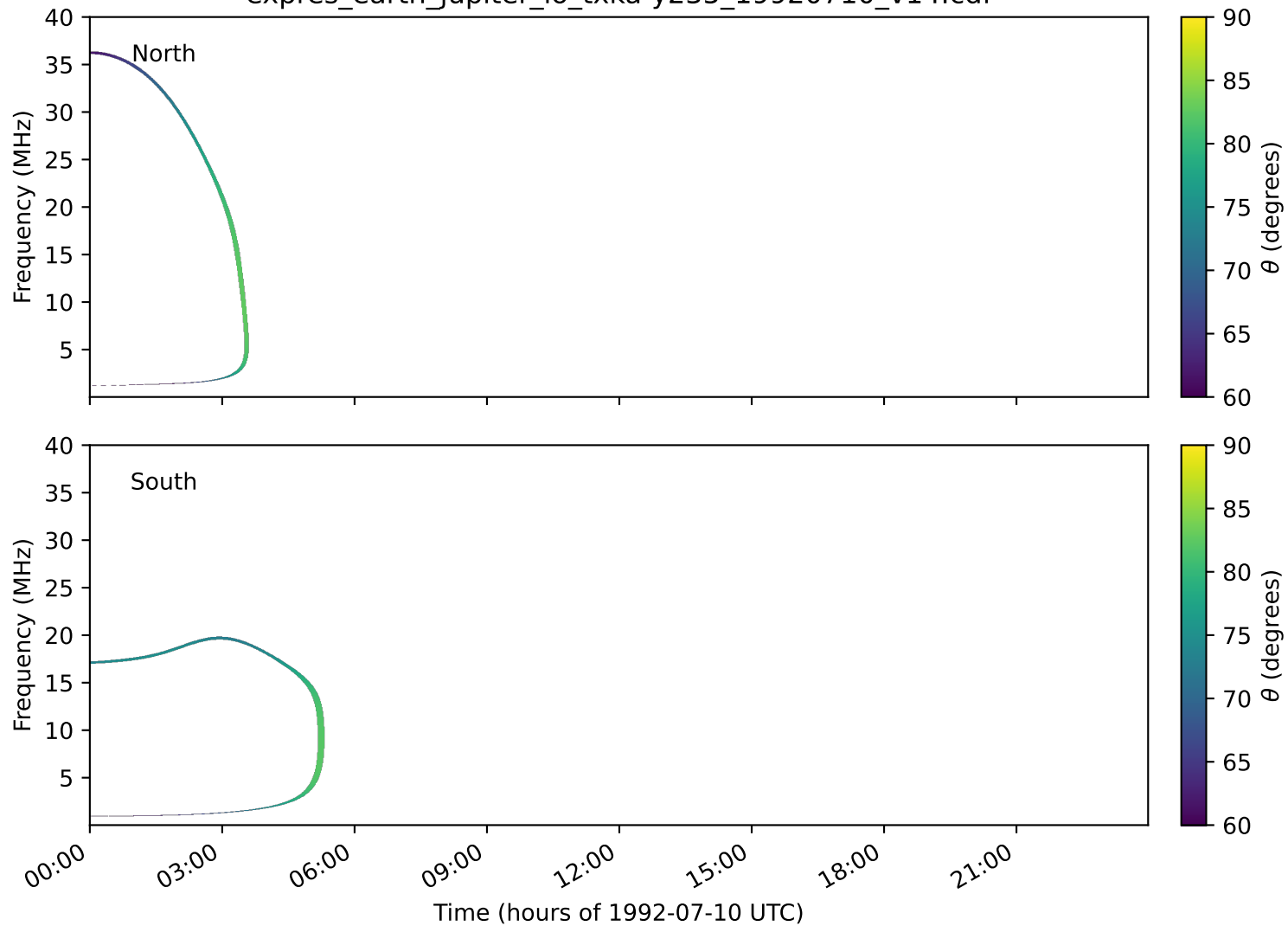
expres_earth_jupiter_io_txka-y235_19920710_v14.cdf
