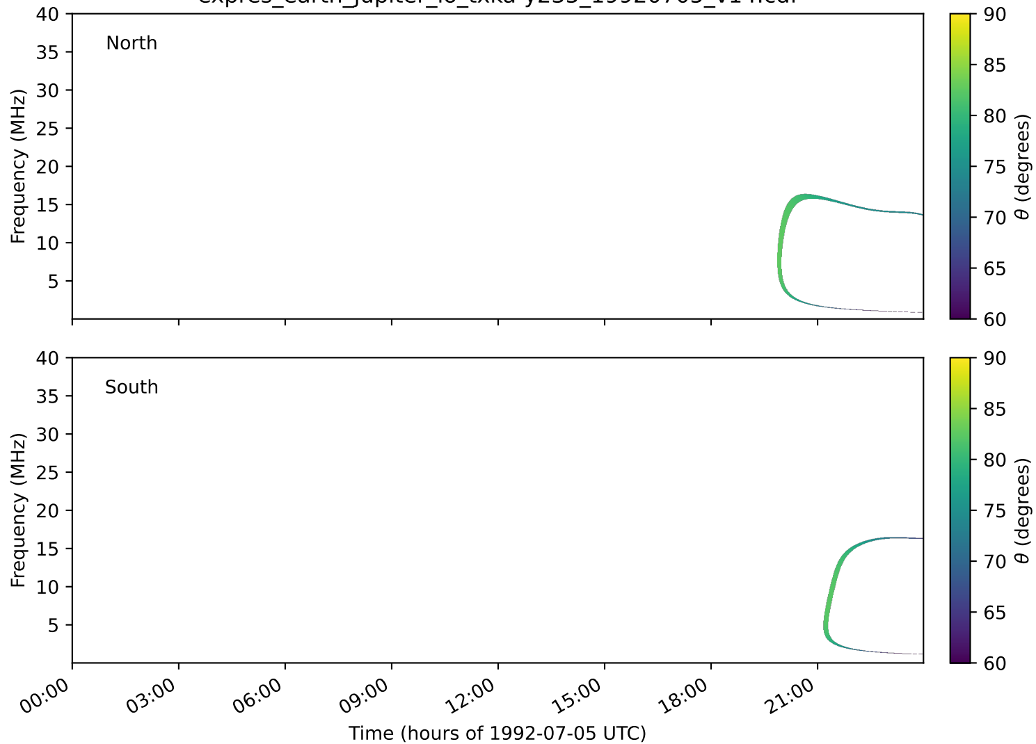
expres_earth_jupiter_io_txka-y235_19920705_v14.cdf
