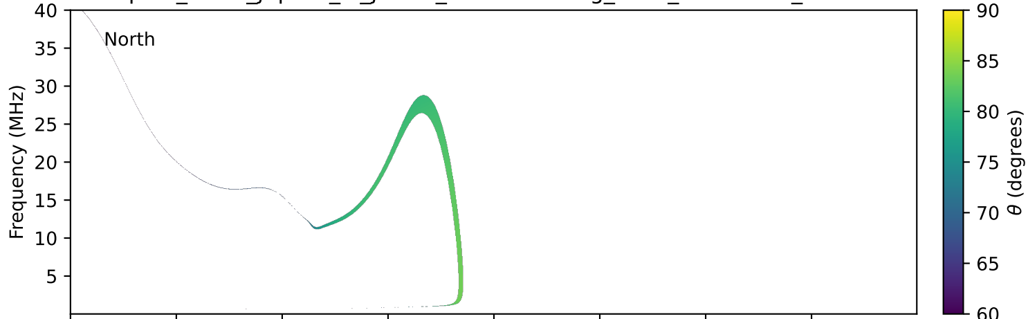
expres_earth_jupiter_io_jrm33_lossc-wid1deg_3kev_19920722_v11.cdf
