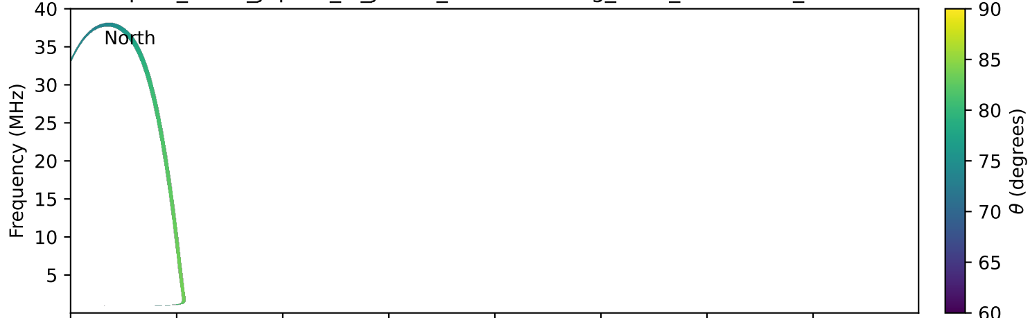
expres_earth_jupiter_io_jrm33_lossc-wid1deg_3kev_19920717_v11.cdf
