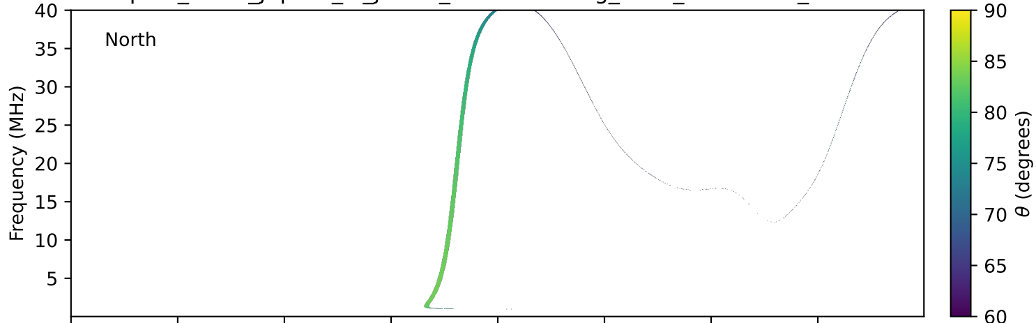
expres_earth_jupiter_io_jrm33_lossc-wid1deg_3kev_19920709_v11.cdf
