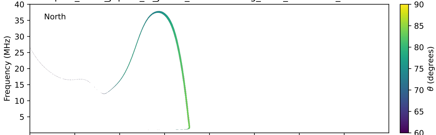
expres_earth_jupiter_io_jrm33_lossc-wid1deg_3kev_19920708_v11.cdf
