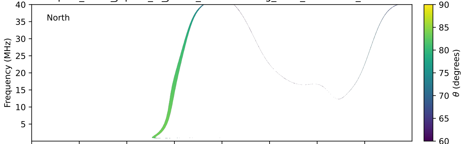
expres_earth_jupiter_io_jrm33_lossc-wid1deg_3kev_19920702_v11.cdf
