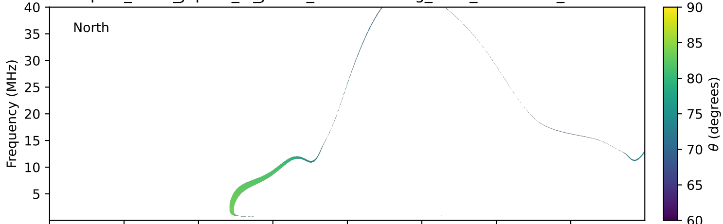
expres_earth_jupiter_io_jrm09_lossc-wid1deg_3kev_19920730_v11.cdf
