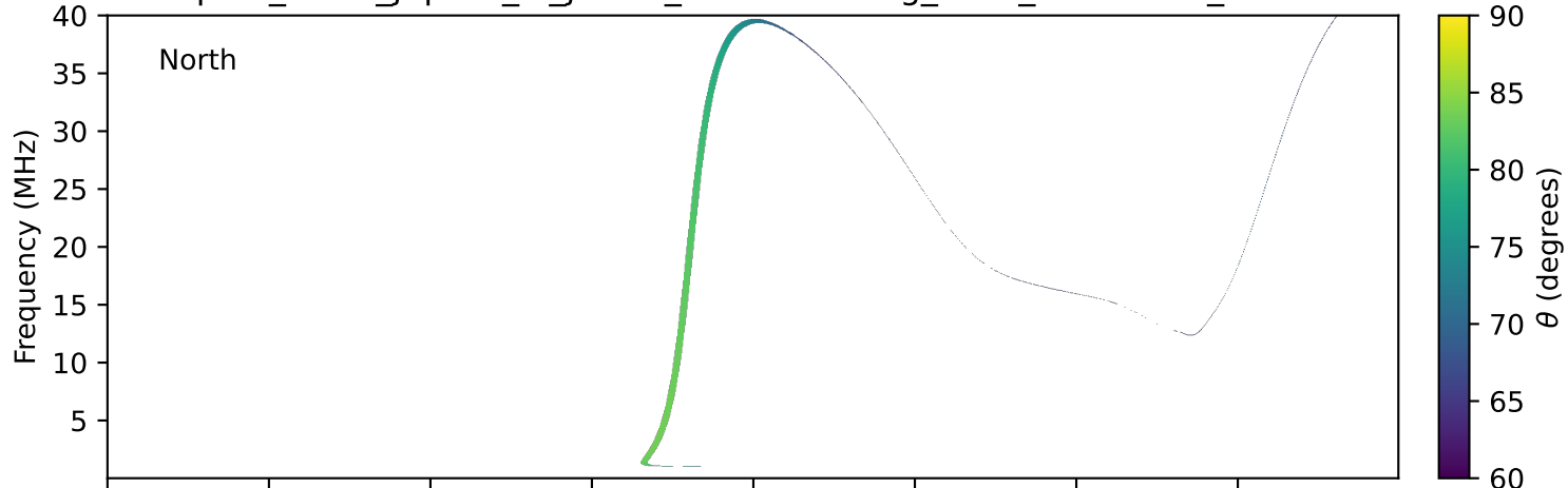
expres_earth_jupiter_io_jrm09_lossc-wid1deg_3kev_19920709_v11.cdf
