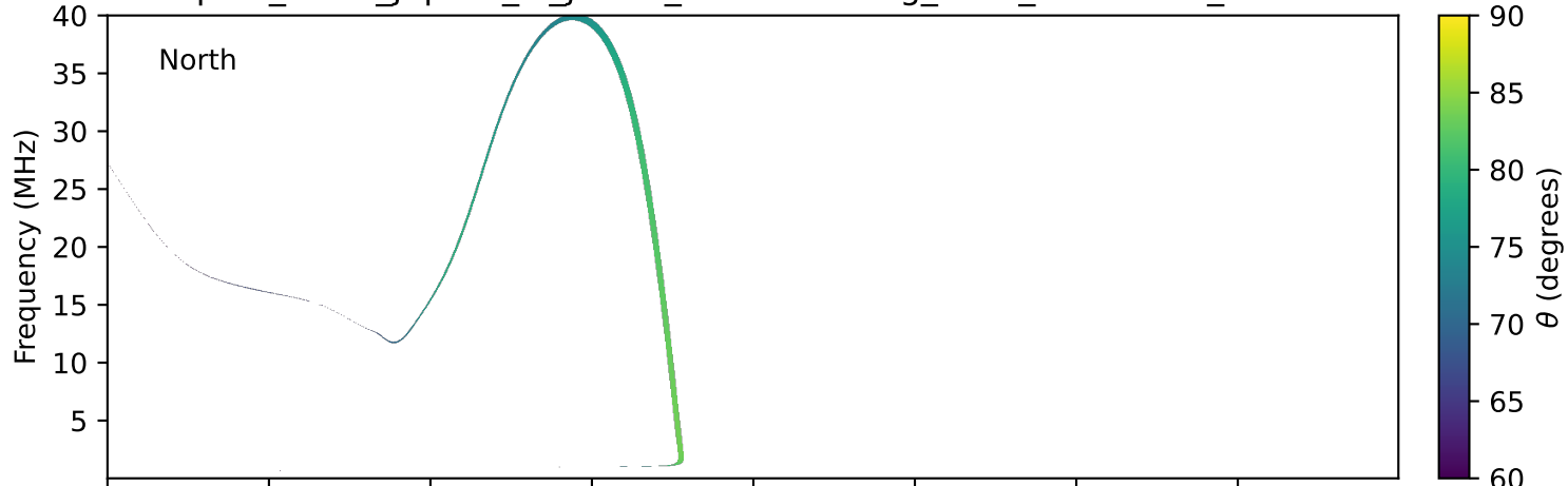
expres_earth_jupiter_io_jrm09_lossc-wid1deg_3kev_19920708_v11.cdf
