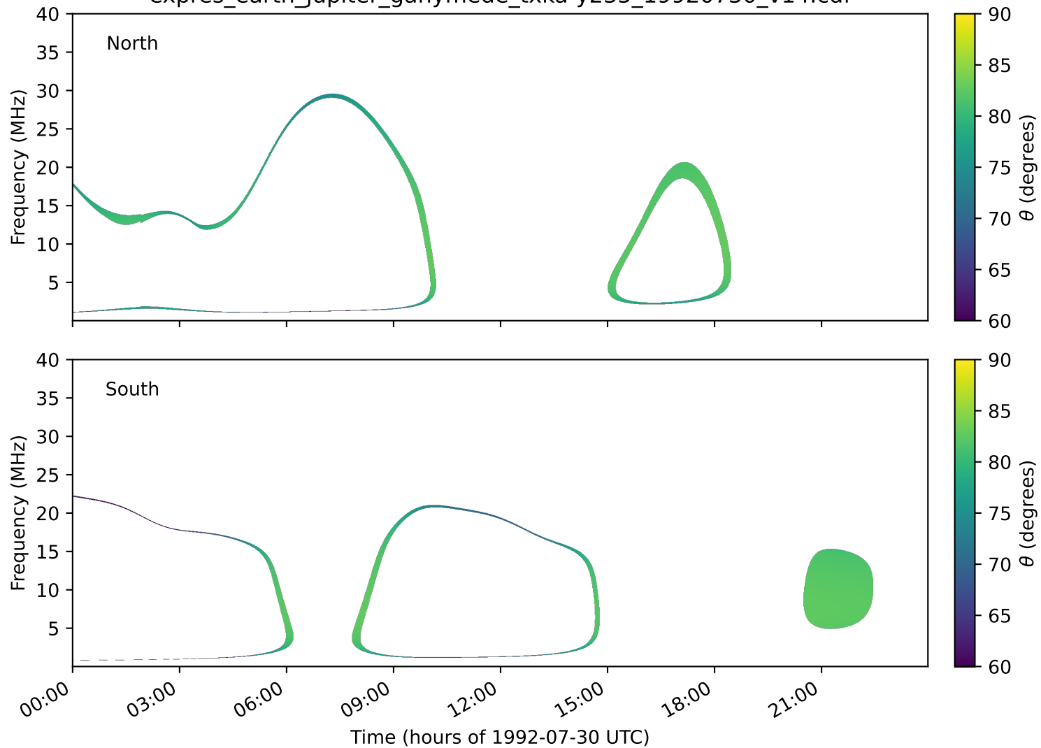
expres_earth_jupiter_ganymede_txka-y235_19920730_v14.cdf
