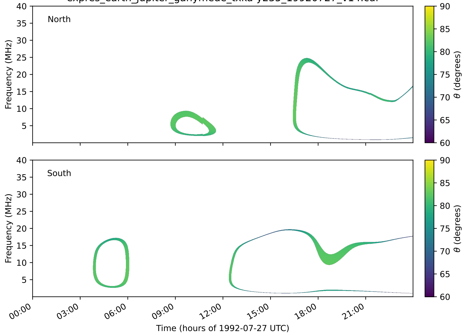
expres_earth_jupiter_ganymede_txka-y235_19920727_v14.cdf
