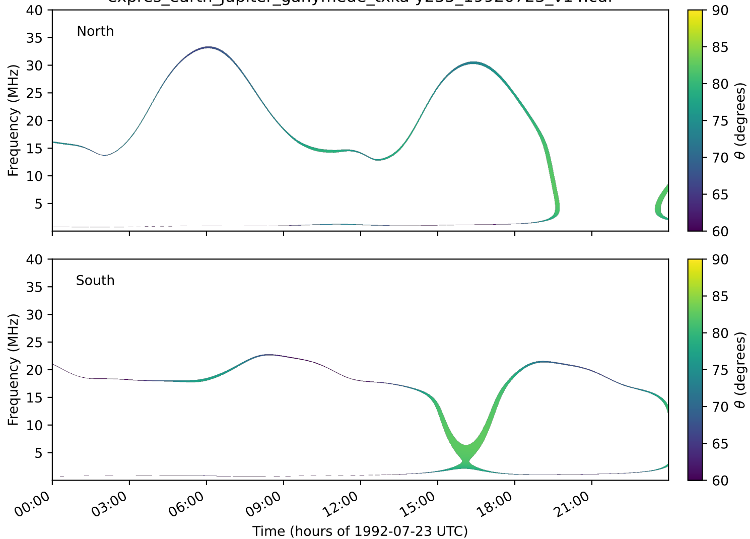
expres_earth_jupiter_ganymede_txka-y235_19920723_v14.cdf
