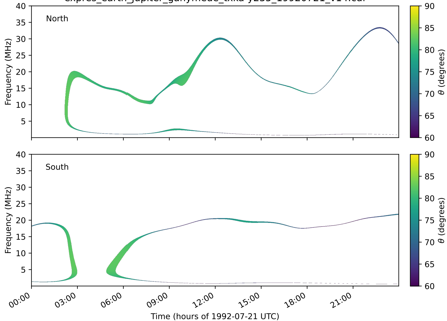
expres_earth_jupiter_ganymede_txka-y235_19920721_v14.cdf
