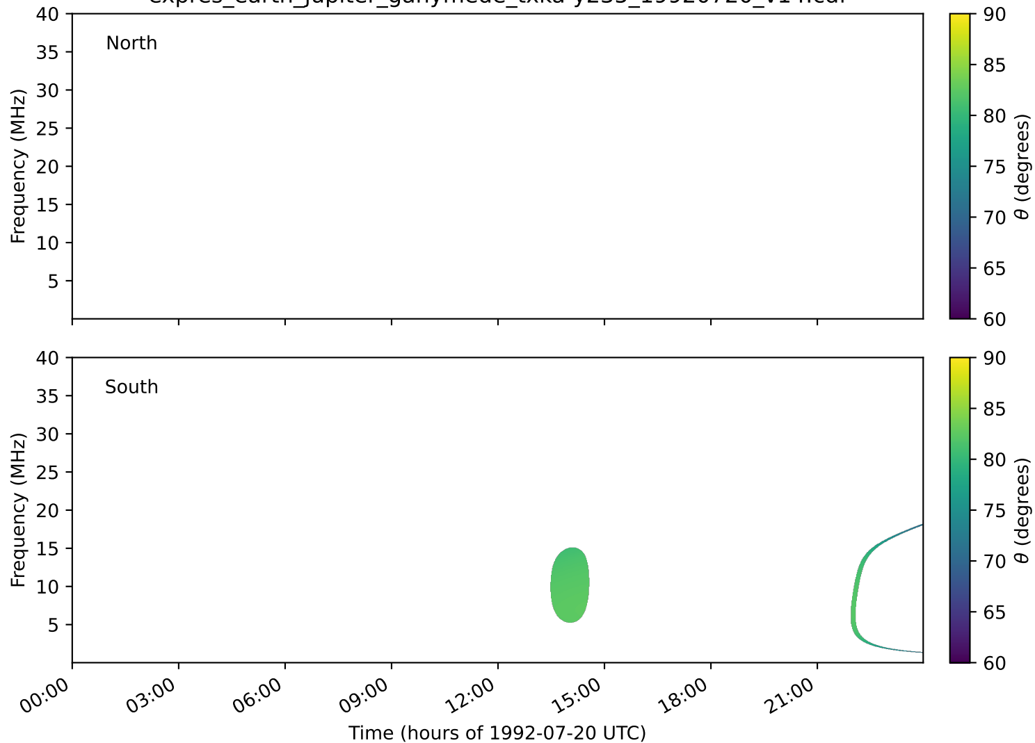
expres_earth_jupiter_ganymede_txka-y235_19920720_v14.cdf
