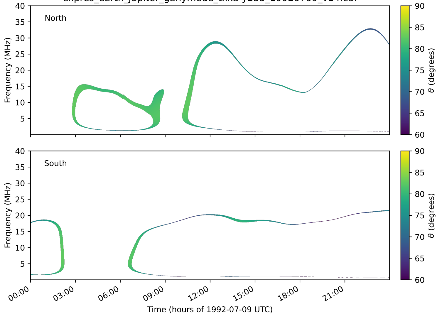
expres_earth_jupiter_ganymede_txka-y235_19920709_v14.cdf
