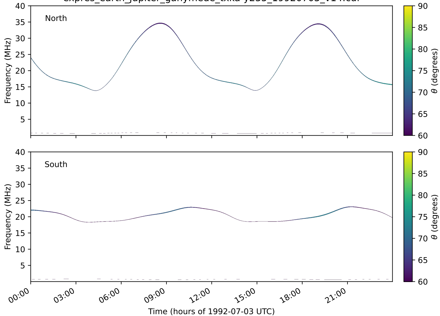
expres_earth_jupiter_ganymede_txka-y235_19920703_v14.cdf
