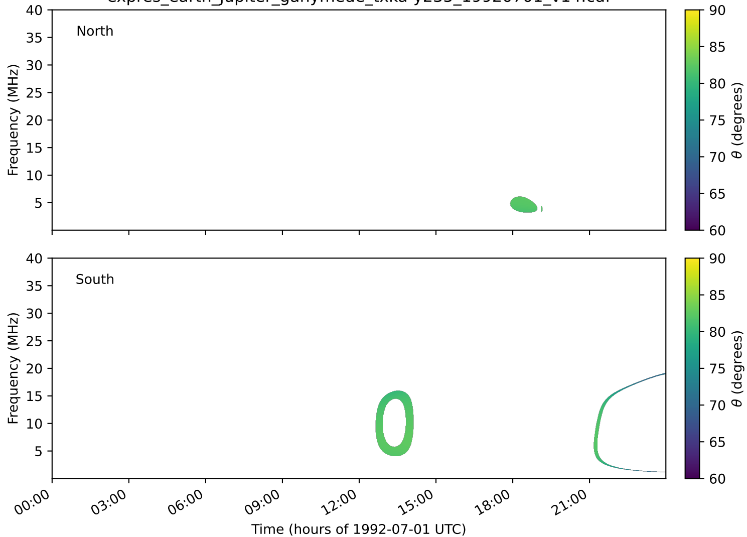
expres_earth_jupiter_ganymede_txka-y235_19920701_v14.cdf
