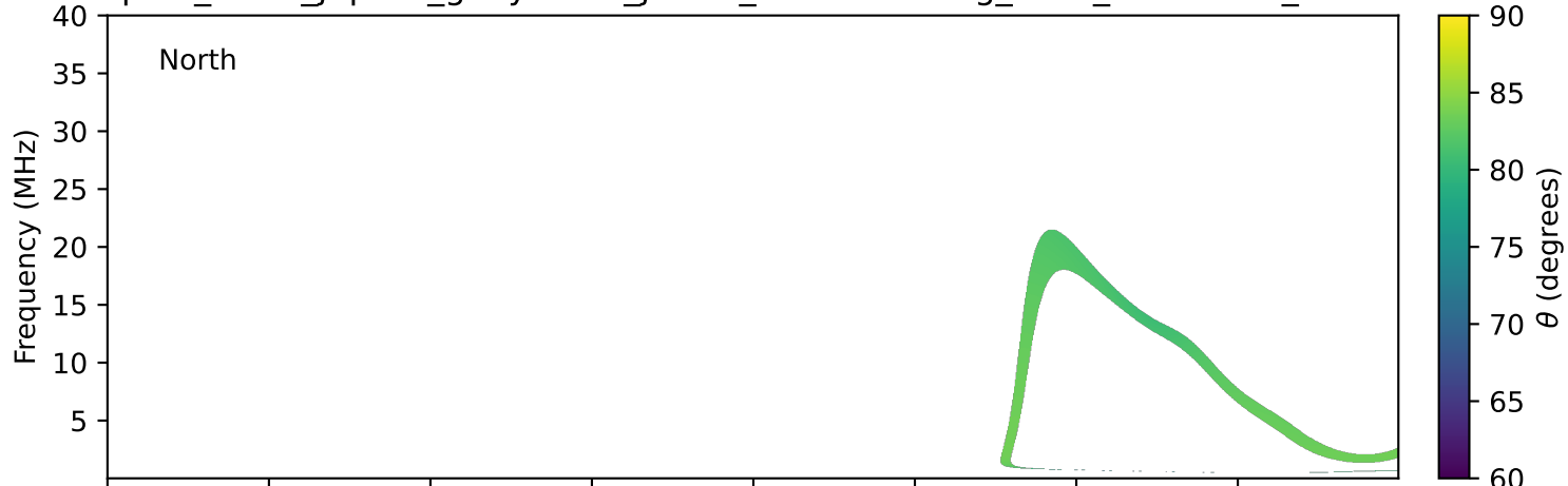
expres_earth_jupiter_ganymede_jrm33_lossc-wid1deg_3kev_19920727_v11.cdf
