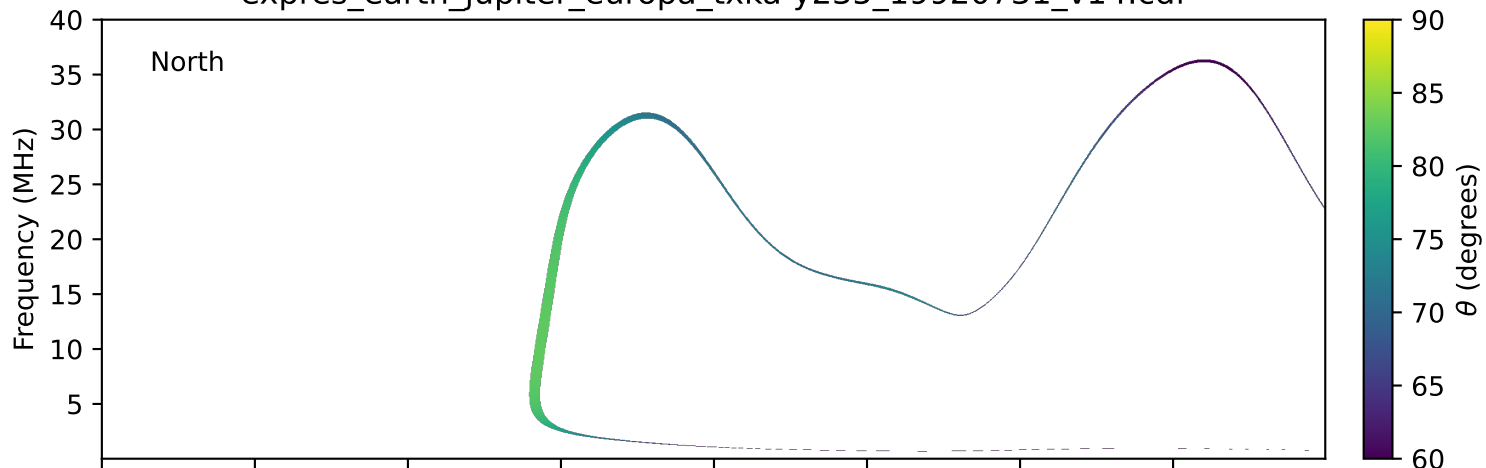
expres_earth_jupiter_europa_txka-y235_19920731_v14.cdf
