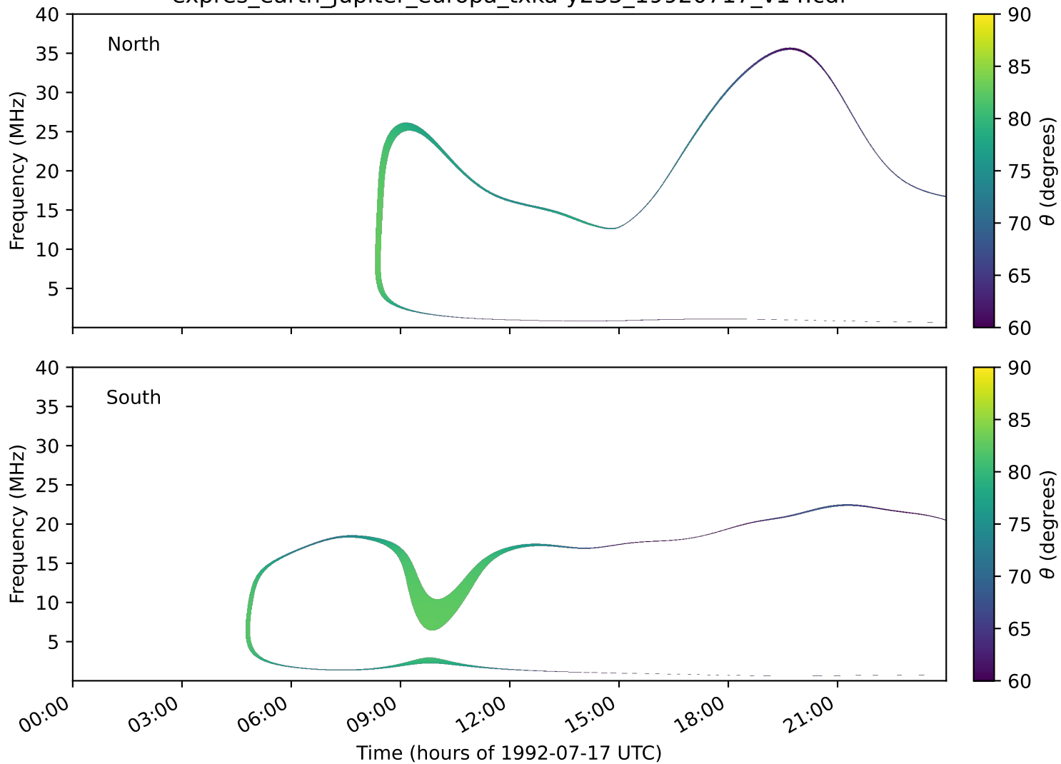
expres_earth_jupiter_europa_txka-y235_19920717_v14.cdf
