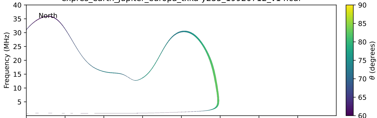
expres_earth_jupiter_europa_txka-y235_19920712_v14.cdf
