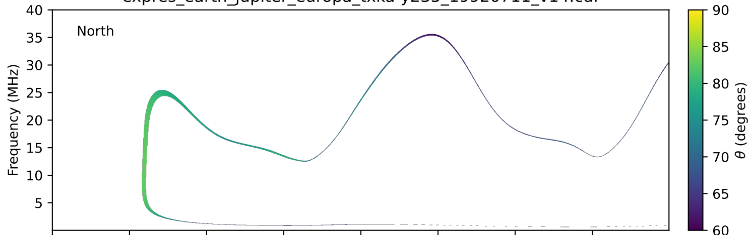
expres_earth_jupiter_europa_txka-y235_19920711_v14.cdf
