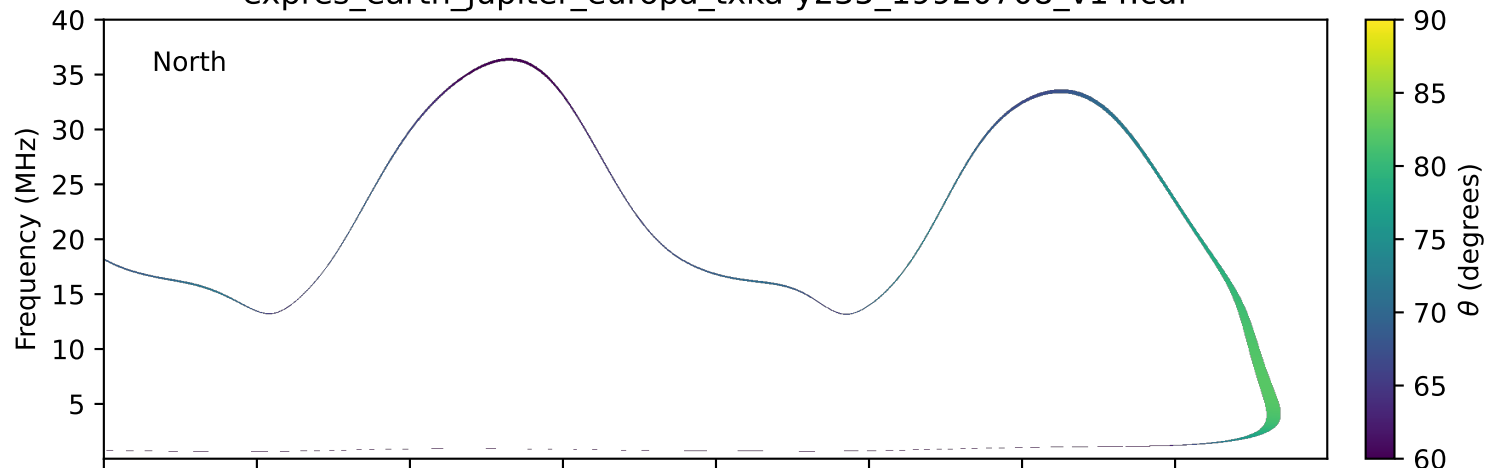
expres_earth_jupiter_europa_txka-y235_19920708_v14.cdf
