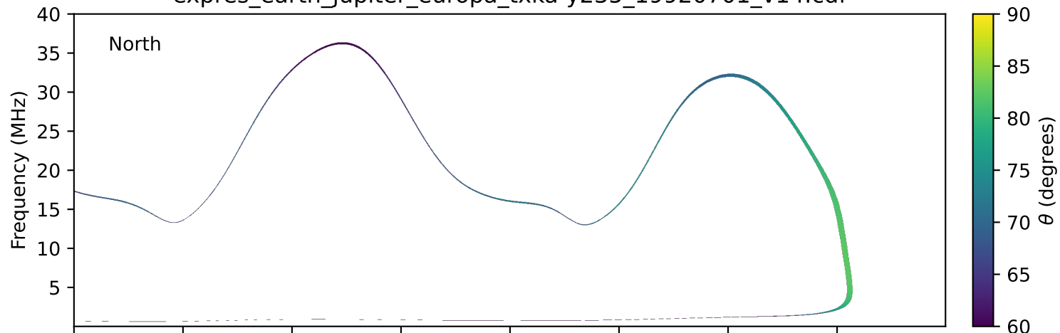
expres_earth_jupiter_europa_txka-y235_19920701_v14.cdf
