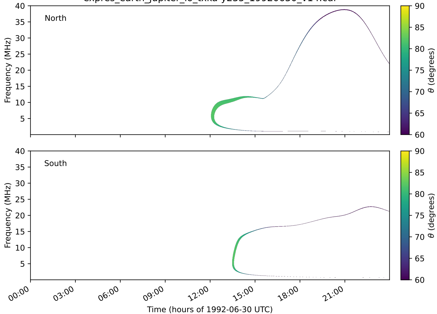
expres_earth_jupiter_io_txka-y235_19920630_v14.cdf
