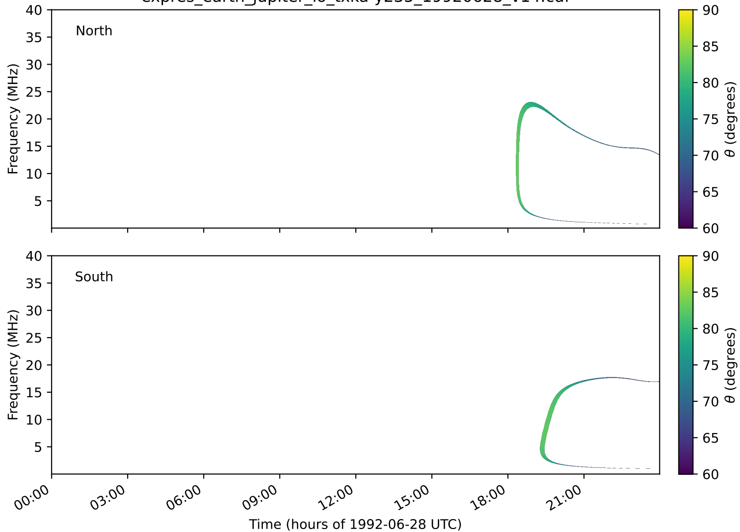
expres_earth_jupiter_io_txka-y235_19920628_v14.cdf
