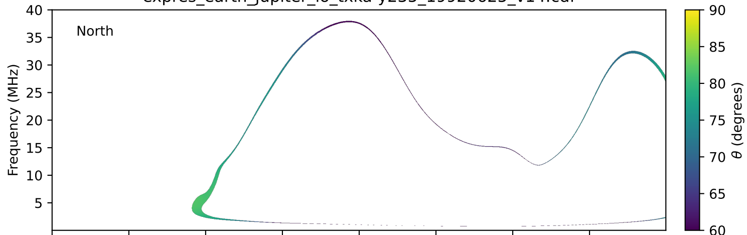
expres_earth_jupiter_io_txka-y235_19920625_v14.cdf
