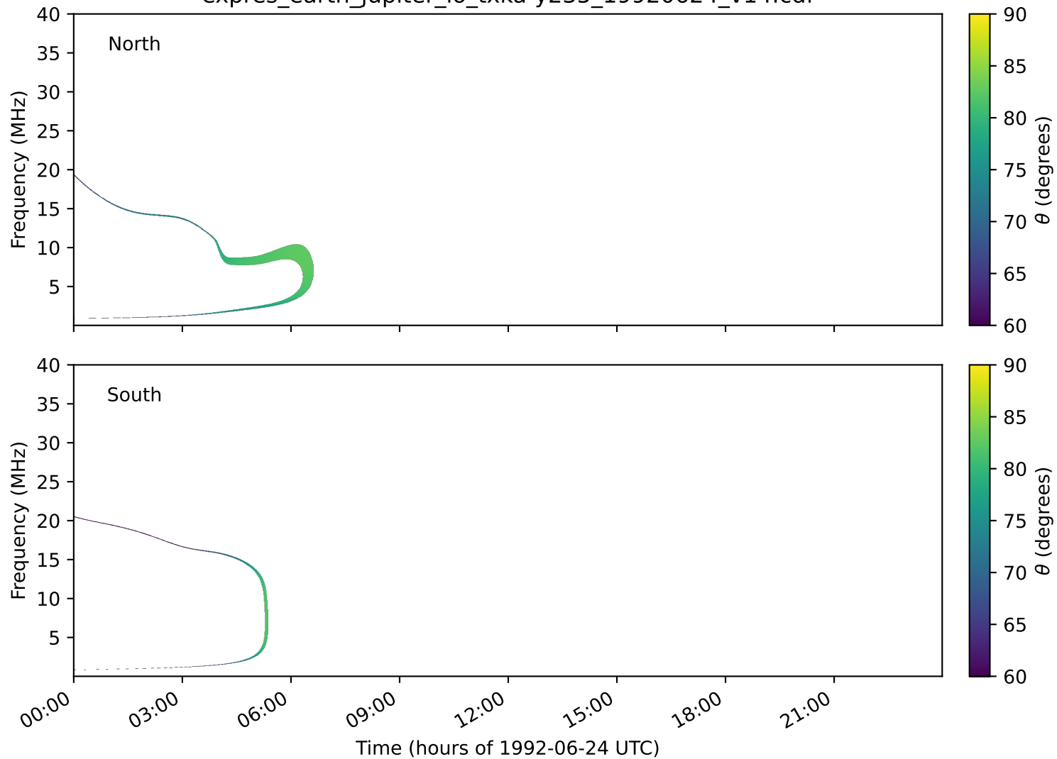
expres_earth_jupiter_io_txka-y235_19920624_v14.cdf
