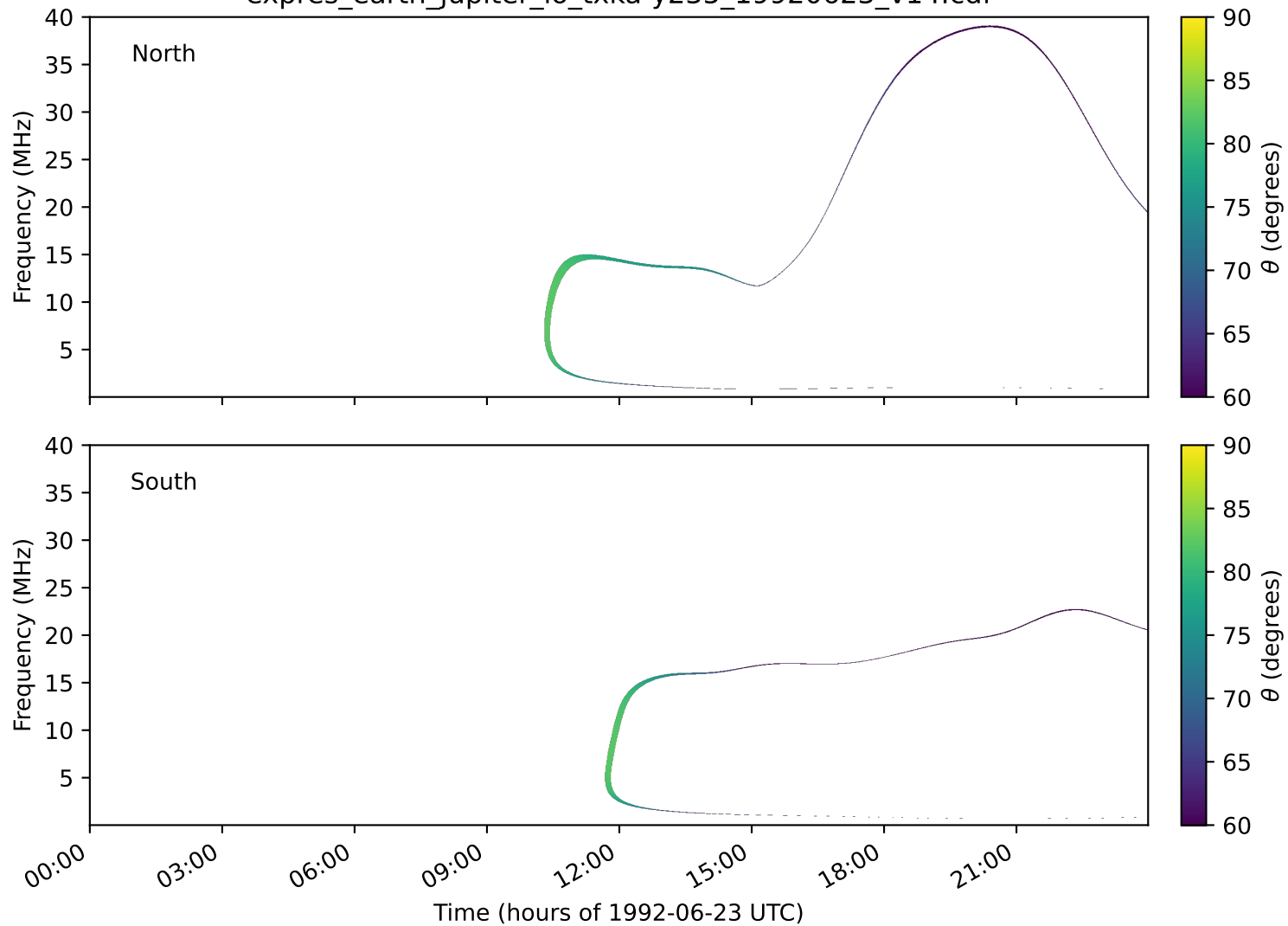
expres_earth_jupiter_io_txka-y235_19920623_v14.cdf
