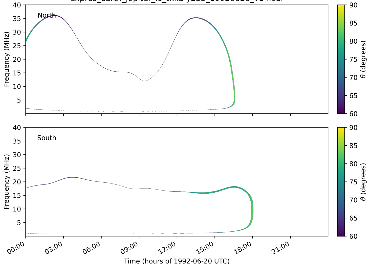
expres_earth_jupiter_io_txka-y235_19920620_v14.cdf
