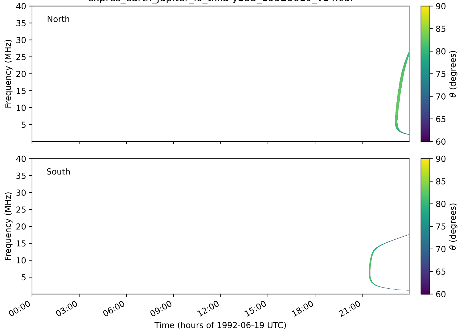
expres_earth_jupiter_io_txka-y235_19920619_v14.cdf
